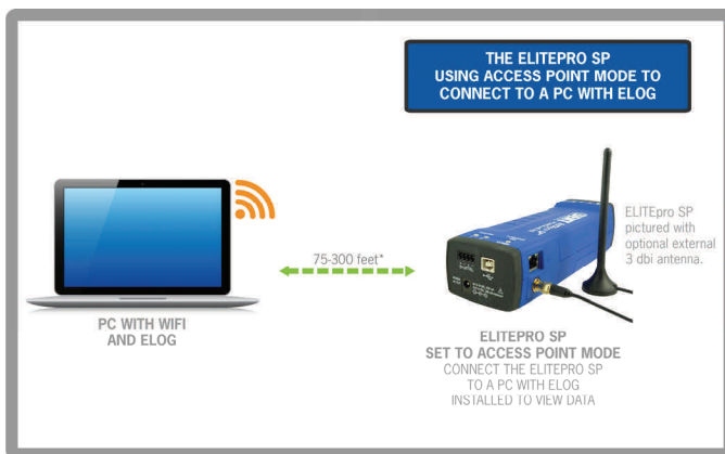
Access Point Mode using ELOG to interface with an ELITEpro SP with Wi-Fi.
